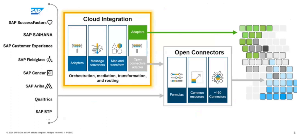
Figure 1.3 Bridge the two worlds of SAP and non-SAP Applications
