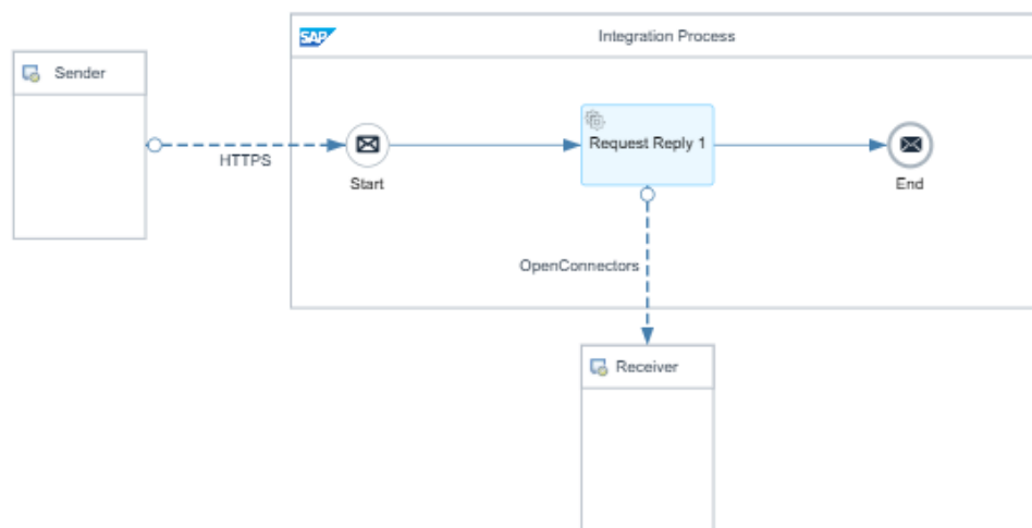
Figure 2.5.3 The designed integration flow is saved and ready to be deploy
