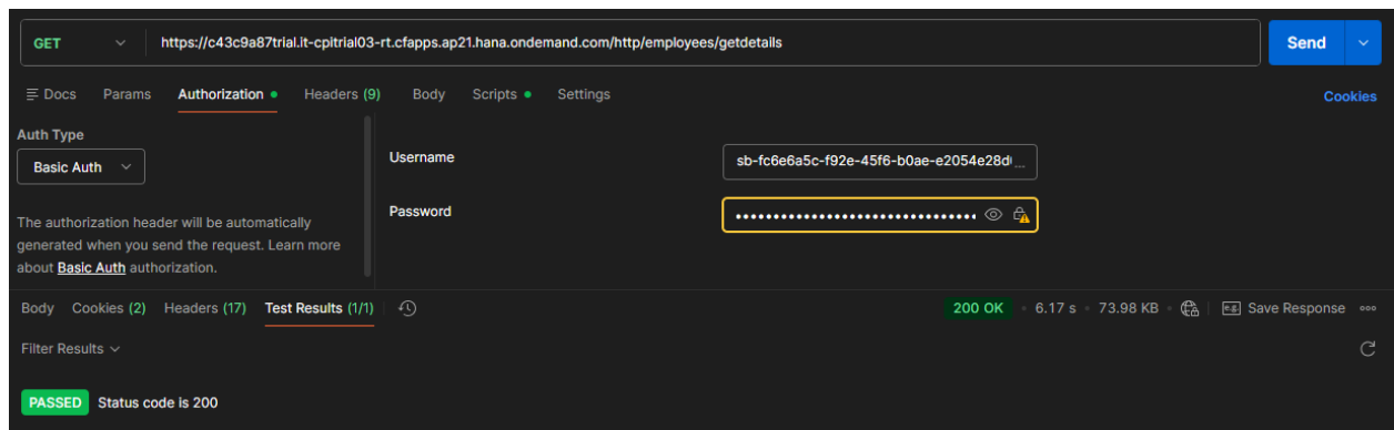
Figure 2.6.2 Tested integration design using Postman API Testing Platform
